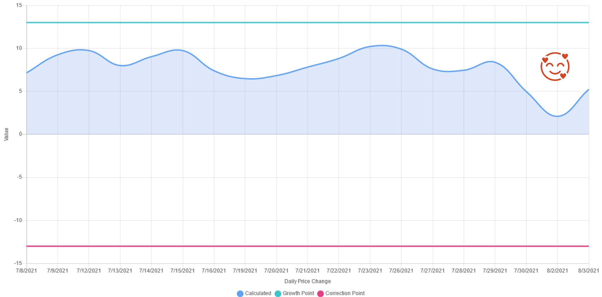
Oscillation vs. Correction
