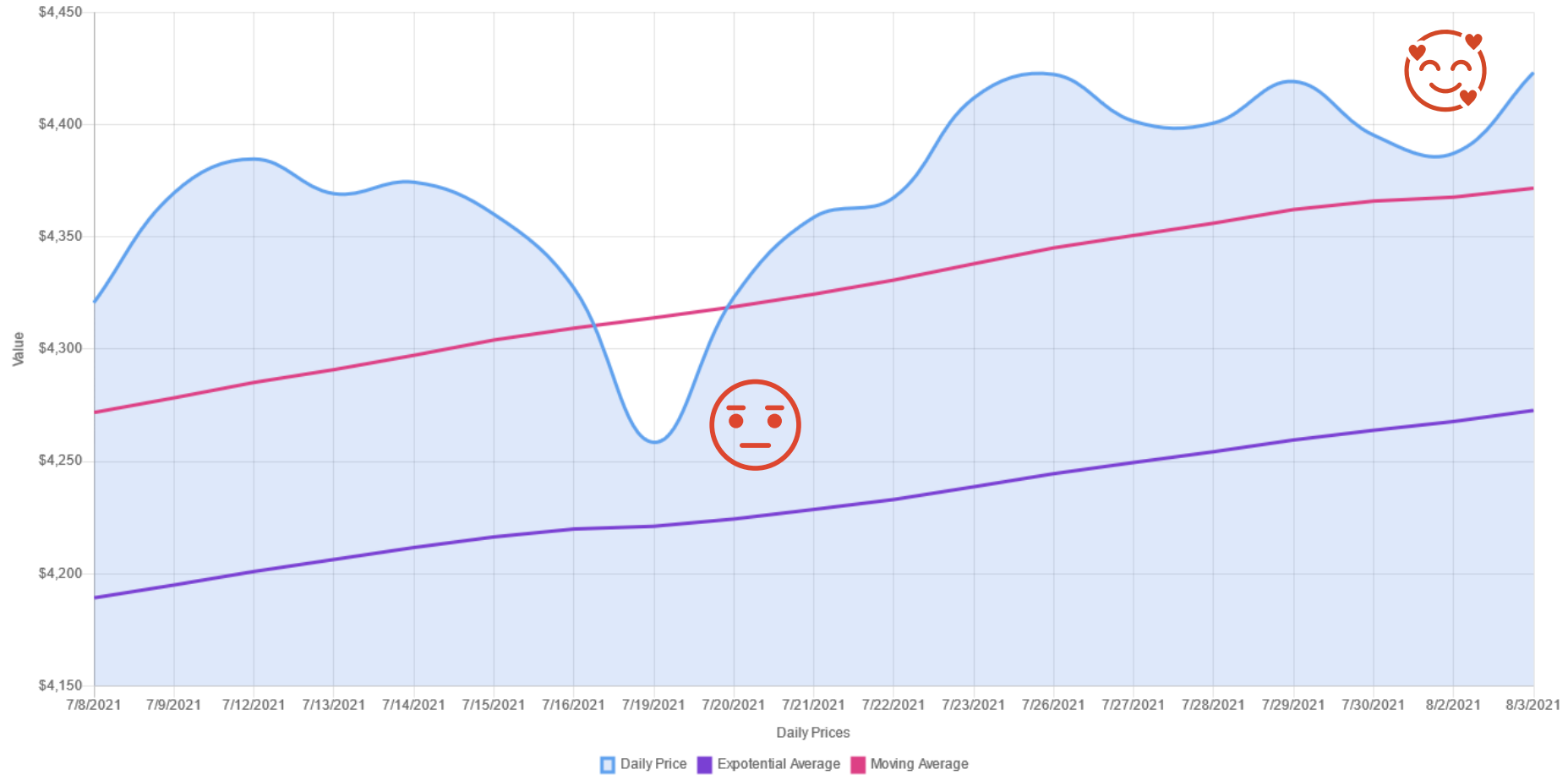
S&P Price, Moving Average and Exponential Average
